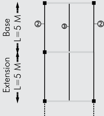
Maximum 25m without windbracings
