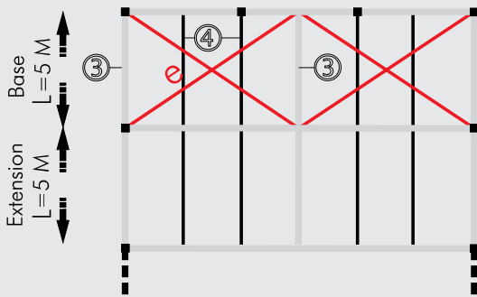
Maximum 25m without windbracings
